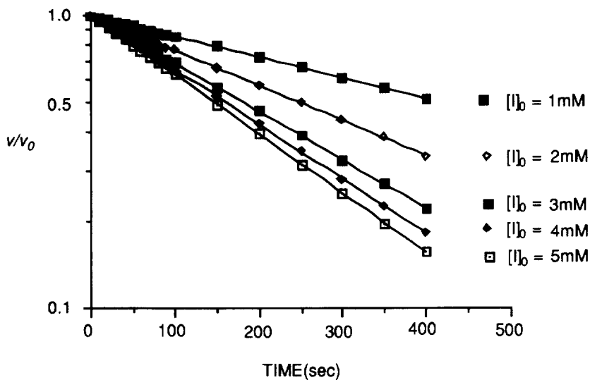
Figure 1. Semilogarithmic plots of the velocity ratio of the substrate hydrolysis after incubating thermolysin with D- 1 of various concentrations vs time of incubation give straight lines with a slope of -k_{\text{obs}} for each inhibitor concentration.
